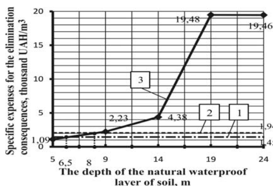
Fig. 6. Graph of the specific costs of pollution elimination against the depth of the waterproof layer of soil: 1 – HIS combined with ID along the two sides of the screen, without the natural waterproof layer (Fig. 2, a); 2 – HIS combined with ID at the perimeter of the storage without natural waterproof layer of (Fig. 2, b); 3 – ID at presence of natural waterproof layer (Fig. 3)
