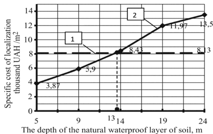
Fig. 4. Graph of the specific localization cost depending on the depth of the waterproof layer of soil:
