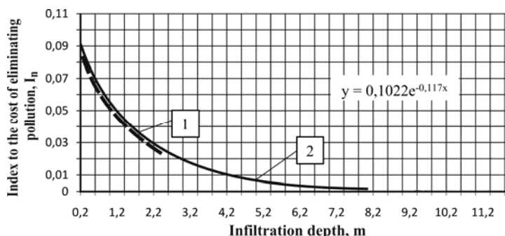
Fig. 5. Graph of dependence l_n of Infiltration depth contaminated water:
