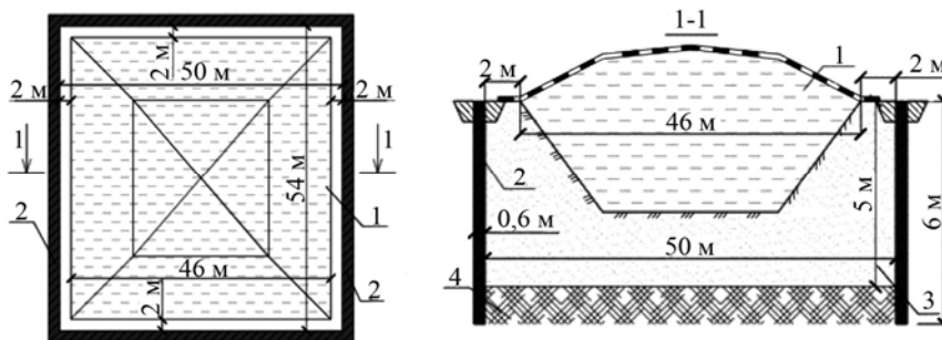
Fig. 3. Localization variant for storage with an waterproof layer of soil:
